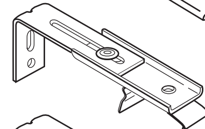
SV-92-29 250 2 7 / 8 - 3 7 / 8 " 73 - 98mm
